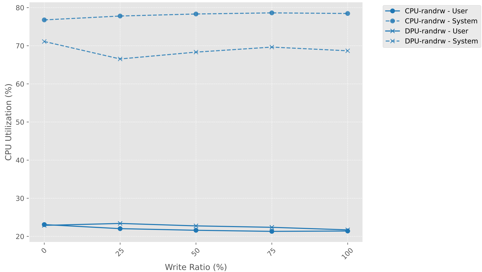
CPU Utilization vs Write Ratio (rwmixwrite-4k-32)
